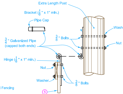
FLOODGATE HINGE AND BRACKET
