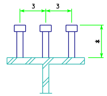
SHEAR STUD DETAILS NOTE: ALL STUDS TO BE 1/2" dia
