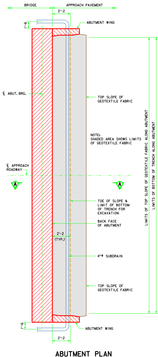
ABUTMENT PLAN
