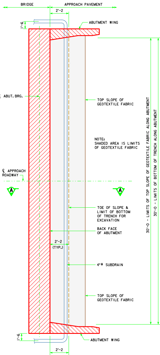
ABUTMENT PLAN WITHOUT WING EXTENSIONS
