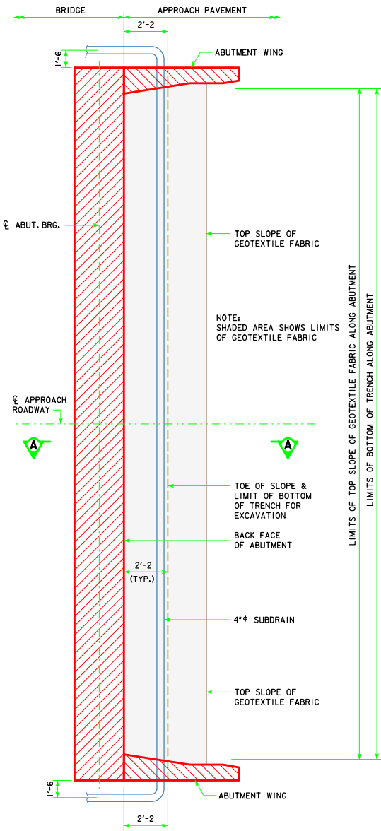
ABUTMENT PLAN WITHOUT WING EXTENSIONS
