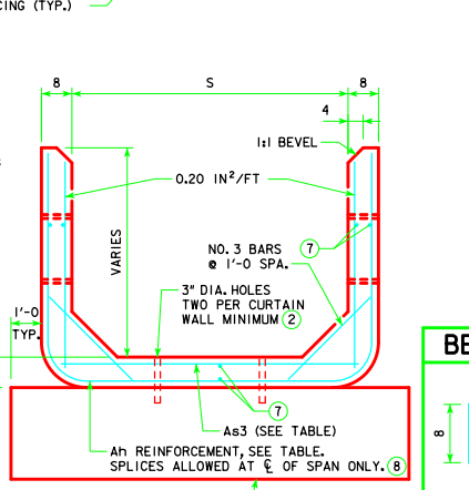
SECTION Z-Z
