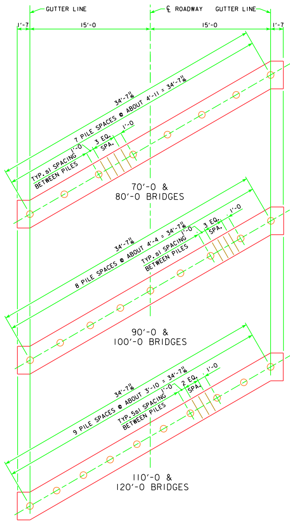
PILE PLAN - 30° SKEW WOOD PILING
