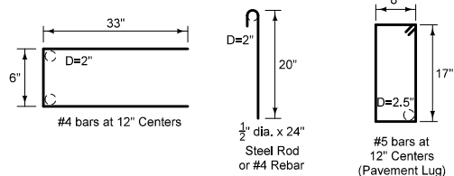
BENT BAR SHAPES
