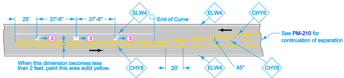
PAINTED CHANNELIZED ISLAND
