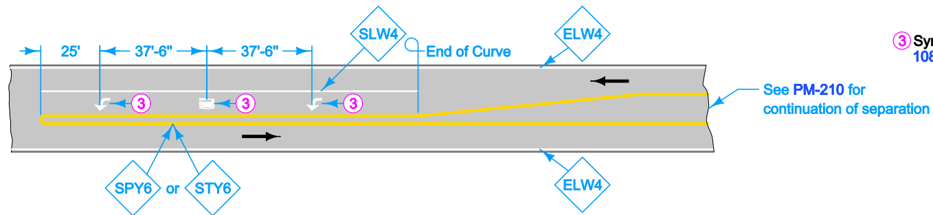
CURBED CHANNELIZED ISLAND
