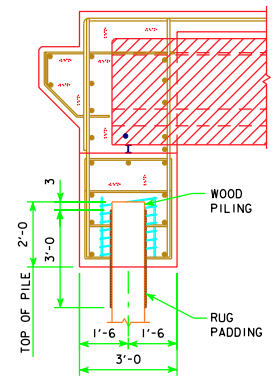
PART SECTION B-B (FOR WOOD PILING)
