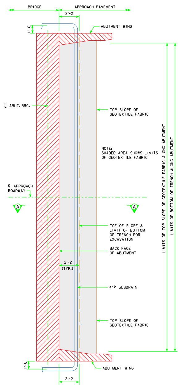
ABUTMENT PLAN WITHOUT WING EXTENSIONS
