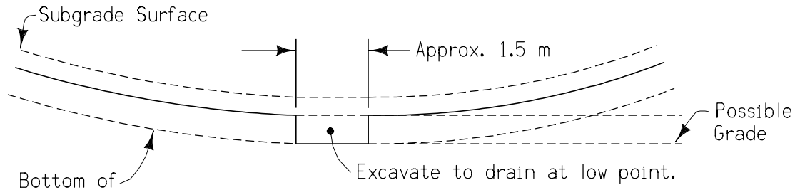
PROFILE VIEW
