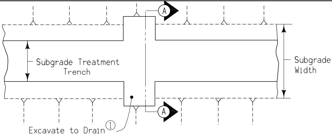
PLAN VIEW
