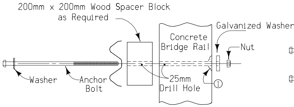
"W" BEAM ATTACHMENT DETAIL
