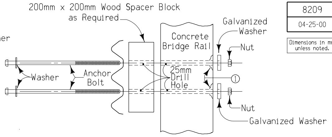
THRIE BEAM ATTACHMENT DETAIL
