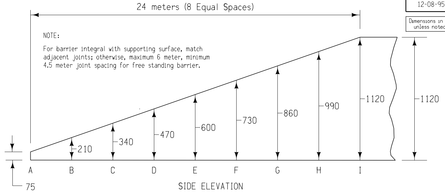
DETAILS OF CONCRETE BARRIER TRANSITION END SECTION (35 MPH or Less)
