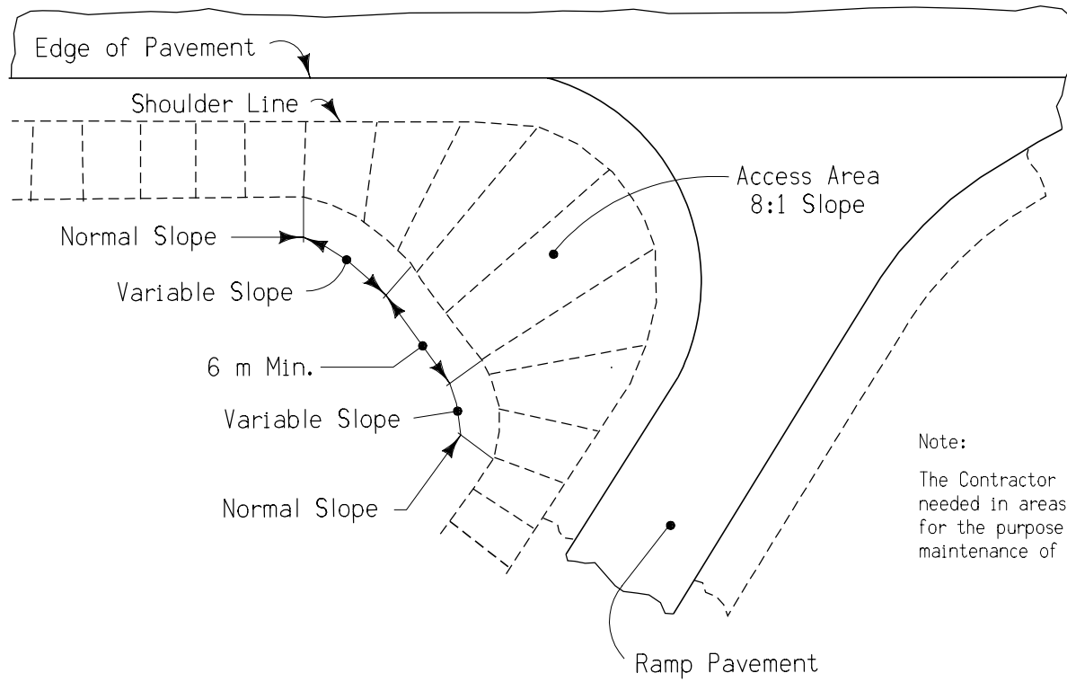
TYPICAL UTILITY ACCESS
