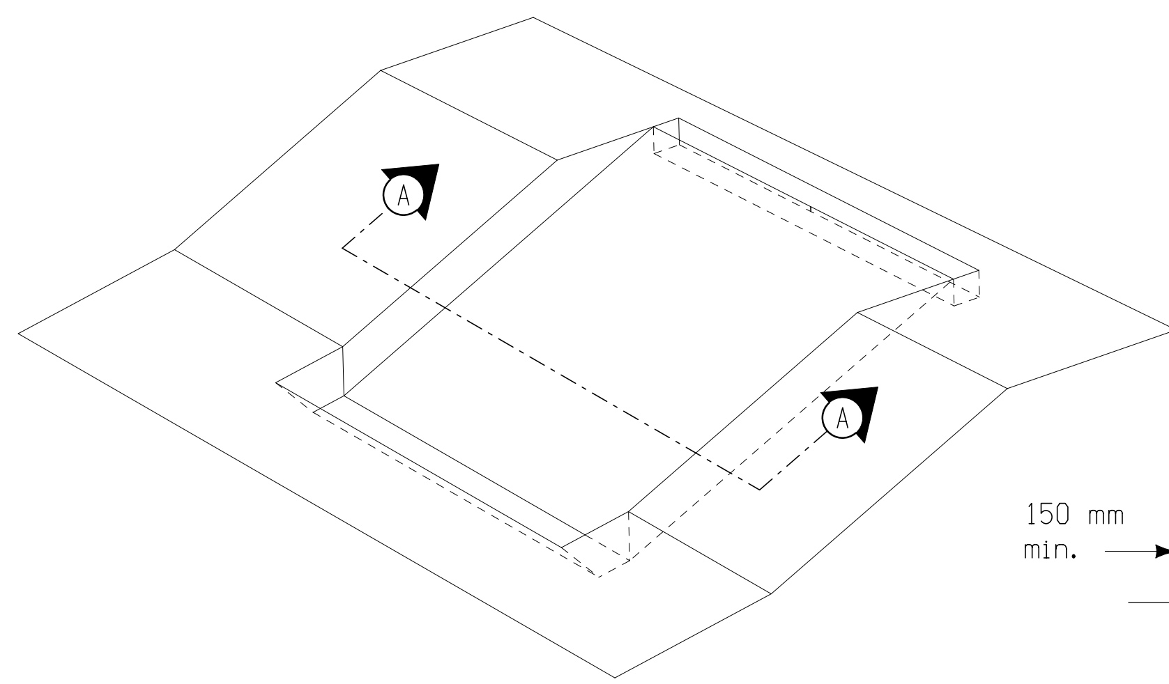
Isometric View
