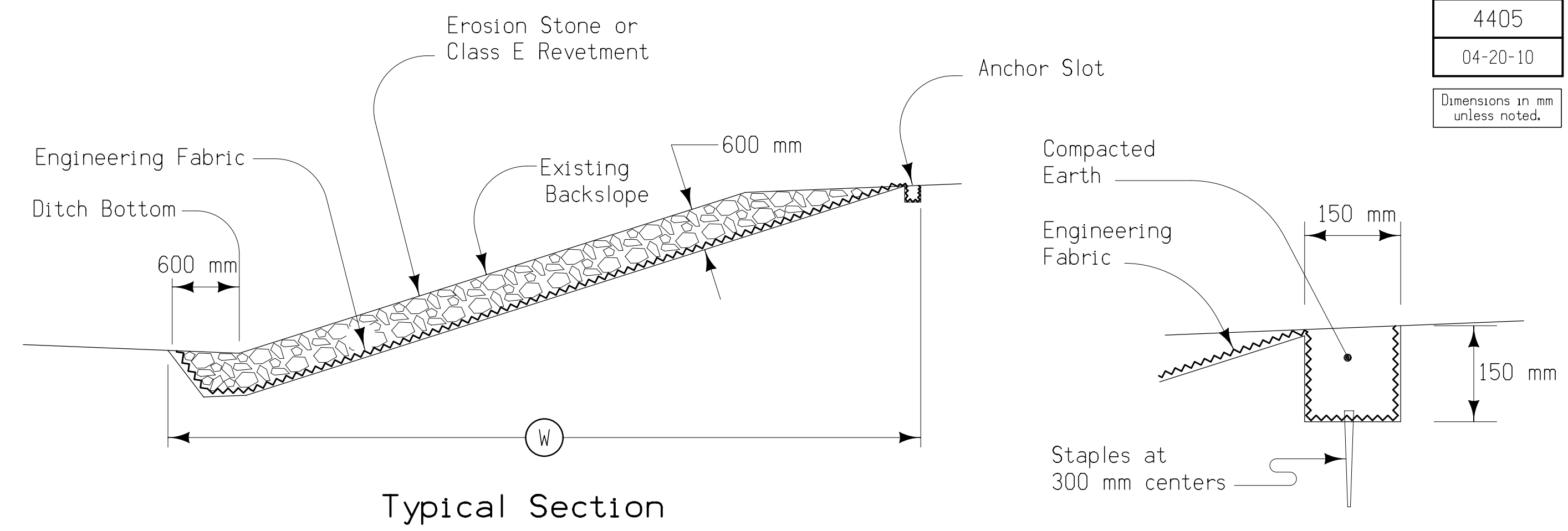
Anchor Slot
