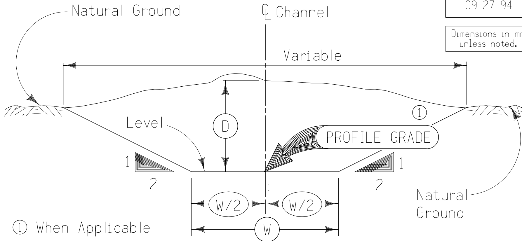
TYPICAL CROSS SECTION TYPE 1 CHANNEL
