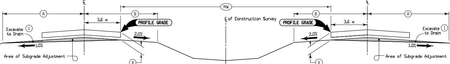
TYPICAL PAVING CROSS SECTION SUBGRADE ADJUSTMENT TO 1% SLOPE 4-LANE DIVIDED ROADWAY
