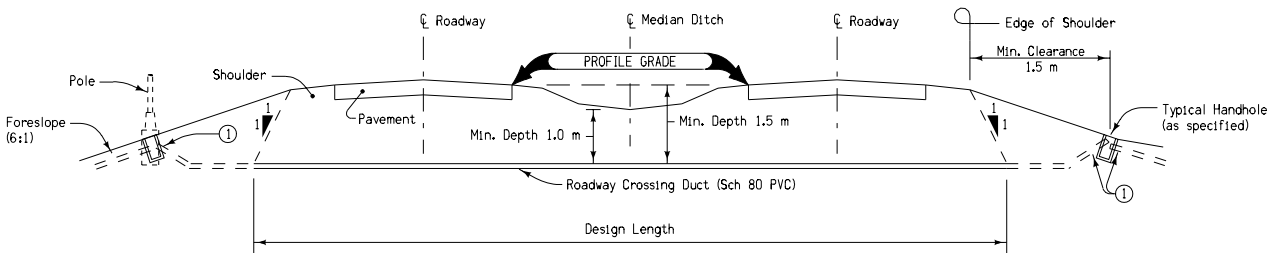
TYPICAL SECTION WHERE FORESLOPES ARE 6:1 OR FLATTER
