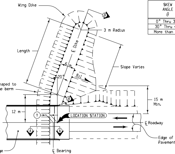
TYPICAL PLAN VIEW OF DIKE CONSTRUCTION AT NON-SKEWED BRIDGE
