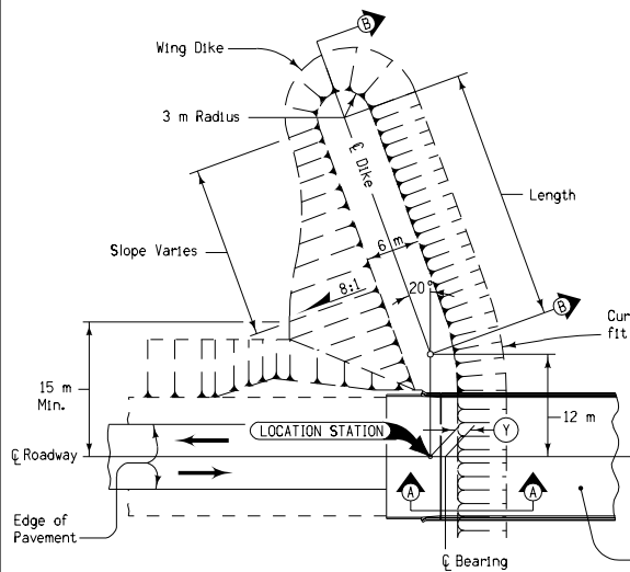
TYPICAL PLAN VIEW OF DIKE CONSTRUCTION AT NON-SKEWED BRIDGE
