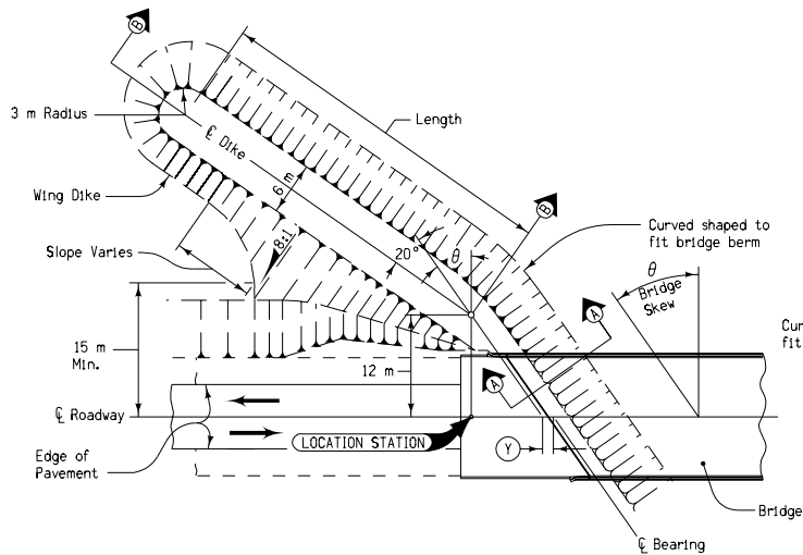
TYPICAL PLAN VIEW OF DIKE CONSTRUCTION AT SKEWED BRIDGE
