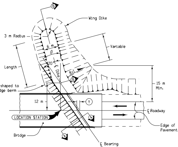
TYPICAL PLAN VIEW OF DIKE CONSTRUCTION AT SKEWED BRIDGE
