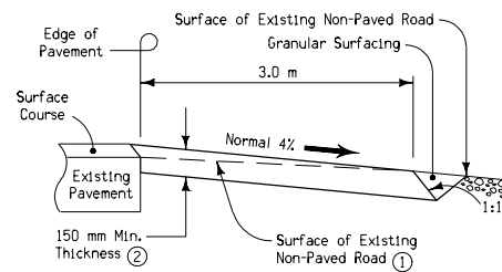
SECTION A-A (FULL THICKNESS FILLET - NON-PAVED ROAD)
