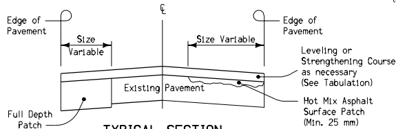
TYPICAL SECTION FULL DEPTH AND SURFACE PATCHES
