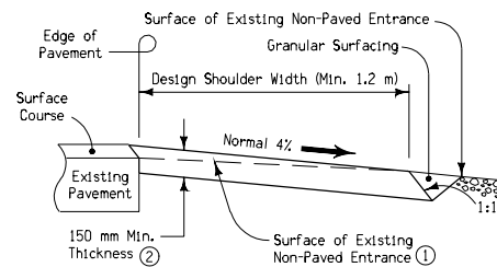
SECTION A-A (FULL THICKNESS FILLET - NON-PAVED ENTRANCE)
