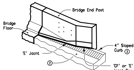
DETAIL 'C' Flared Bridge End Post
