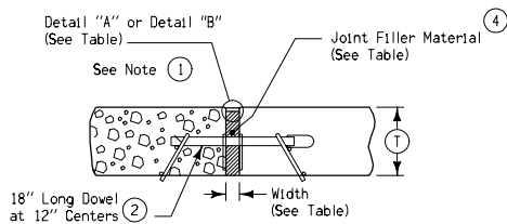
'ED', 'EE', 'EF' DOWELED EXPANSION JOINT
