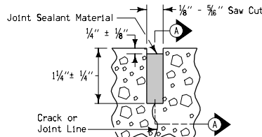
DETAIL "B" (Sawcut formed by approved early concrete saving equipment)
