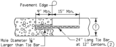
See Note ⑤ 'RT' ABUTTING PAVEMENT JOINT RIGID TIE
