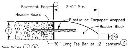
See Notes ⑤ ⑥ 'HT' HEADER JOINT (END RIGID PAVEMENT)
