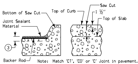
'C' JOINT IN CURB
