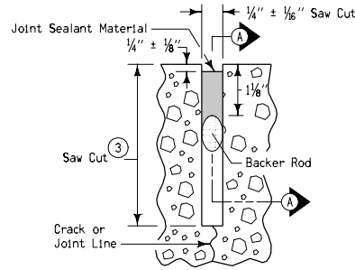
DETAIL "A" (Sawcut formed by conventional concrete saving equipment)
