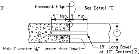
See Notes ⑤ ⑥ 'RD' ABUTTING PAVEMENT JOINT
